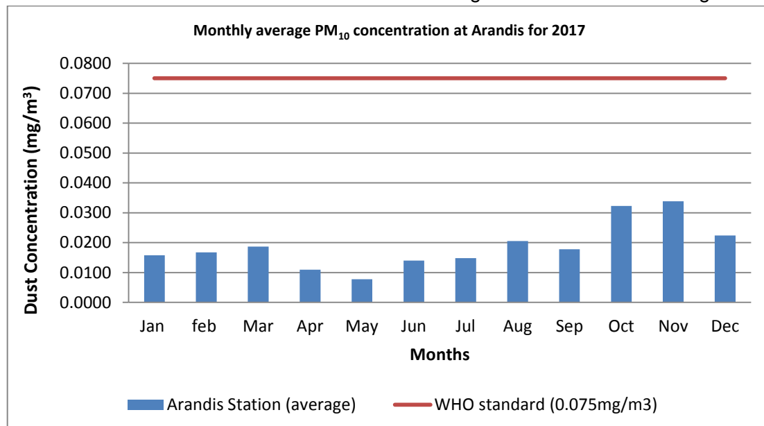
Figure 4.4: Dust concentrations measured in Arandis 2017
